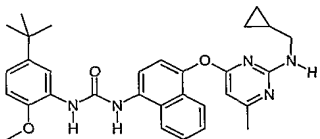
1-(5-tert-Butyl-2-methoxy-phenyl)-3-{4-[2-(cyclopropylmethyl-amino)-6-methyl-pyrimidin-4-yloxy]-naphthalen-1-yl}-urea;
